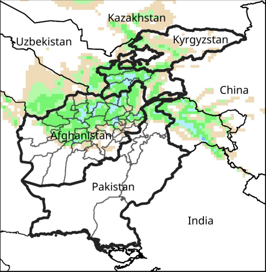
Daily Precip. Forecast for Jan 29, 2025
