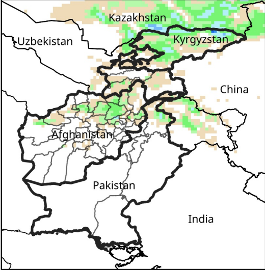
Daily Precip. Forecast for Jan 30, 2025
