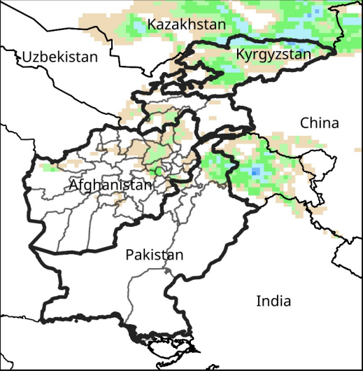
Daily Precip. Forecast for Jan 30, 2025
