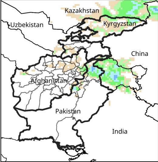
Daily Precip. Forecast for Jan 31, 2025
