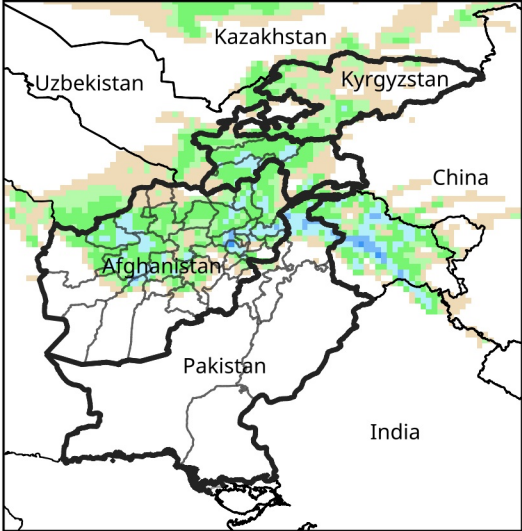
Daily Precip. Forecast for Feb 1, 2025
