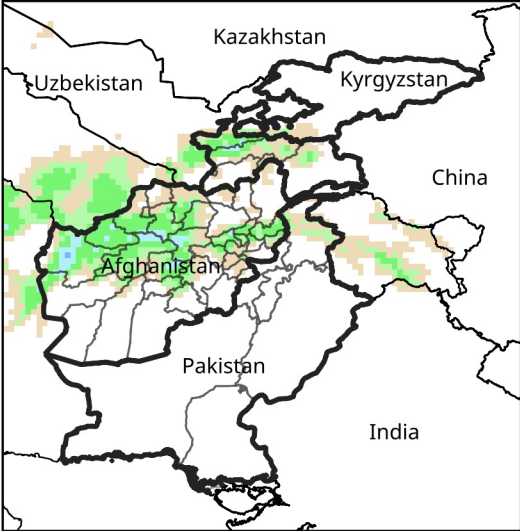
Daily Precip. Forecast for Jan 31, 2025
