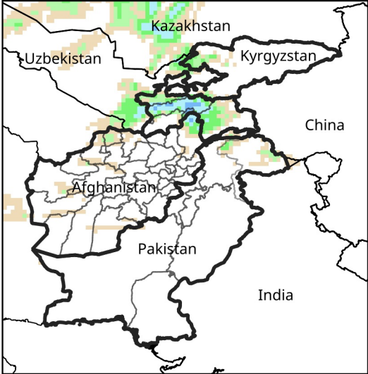
Daily Precip. Forecast for Feb 17, 2025
