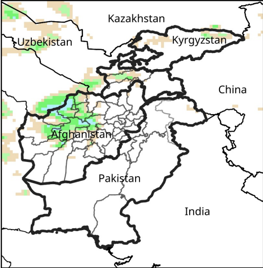
Daily Precip. Forecast for Feb 16, 2025
