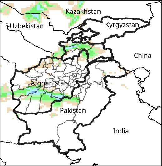
Daily Precip. Forecast for Feb 17, 2025
