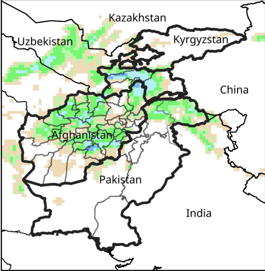
Daily Precip. Forecast for Feb 18, 2025
