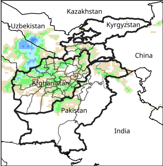
Daily Precip. Forecast for Feb 21, 2025
