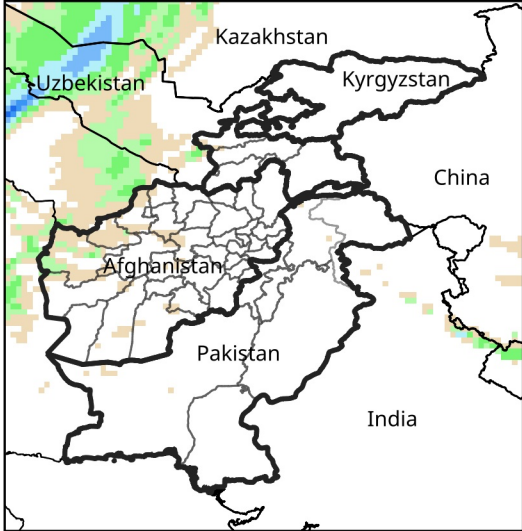
Daily Precip. Forecast for Feb 26, 2025
