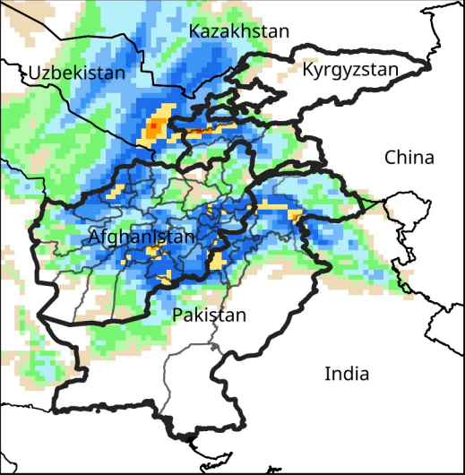
Daily Precip. Forecast for Feb 25, 2025
