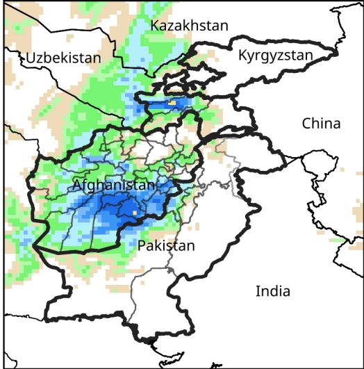
Daily Precip. Forecast for Feb 27, 2025
