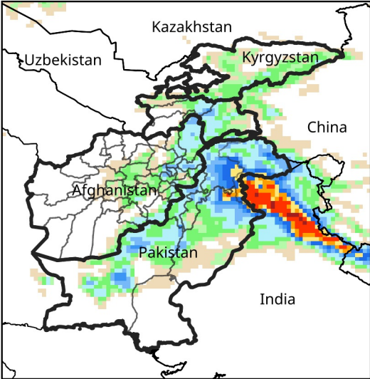
Daily Precip. Forecast for Mar 2, 2025
