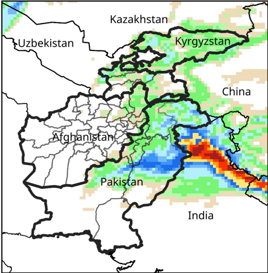
Daily Precip. Forecast for Mar 3, 2025
