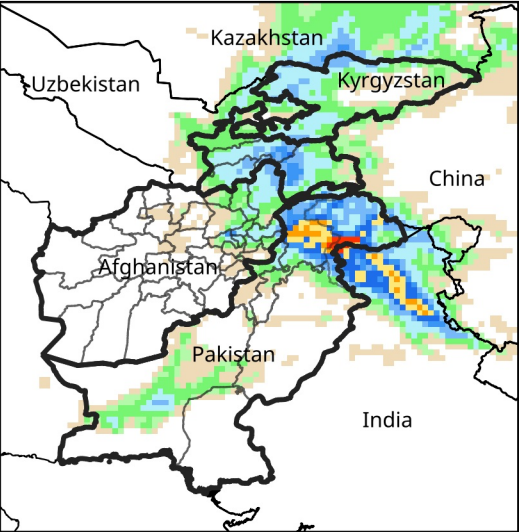
Daily Precip. Forecast for Mar 1, 2025
