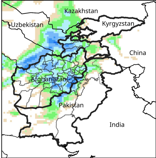
Daily Precip. Forecast for Mar 5, 2025
