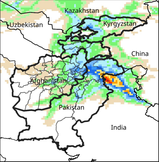
Daily Precip. Forecast for Mar 3, 2025
