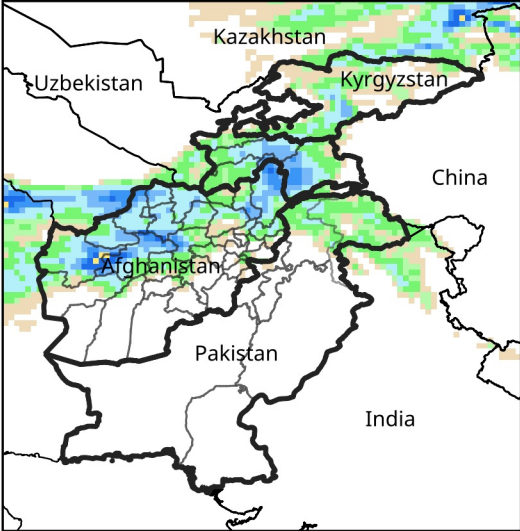
Daily Precip. Forecast for Mar 12, 2025
