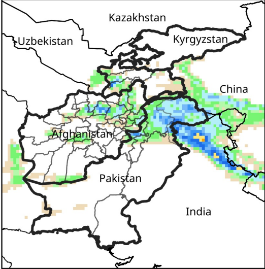
Daily Precip. Forecast for Mar 13, 2025
