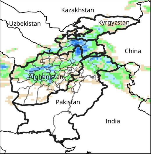
Daily Precip. Forecast for Mar 11, 2025
