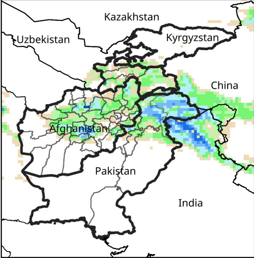
Daily Precip. Forecast for Mar 12, 2025
