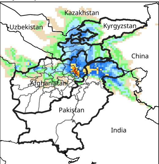
Daily Precip. Forecast for Mar 27, 2025
