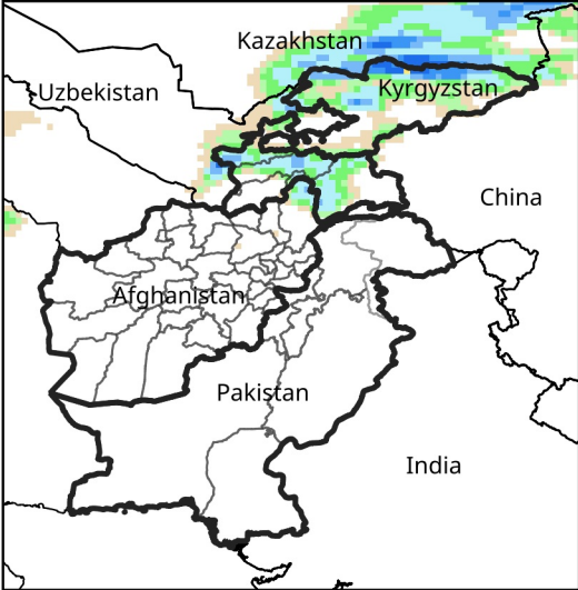
Daily Precip. Forecast for Apr 8, 2025
