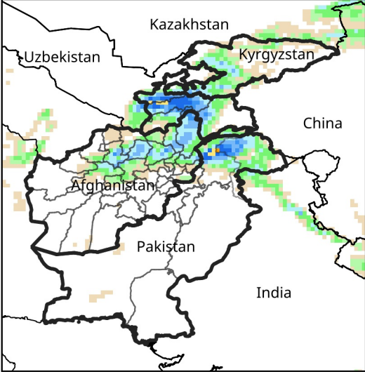
Daily Precip. Forecast for Apr 8, 2025
