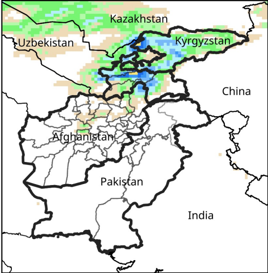
Daily Precip. Forecast for Apr 9, 2025
