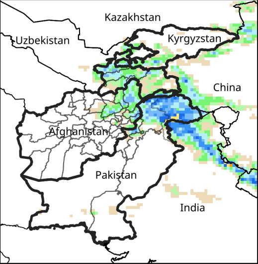
Daily Precip. Forecast for Apr 10, 2025
