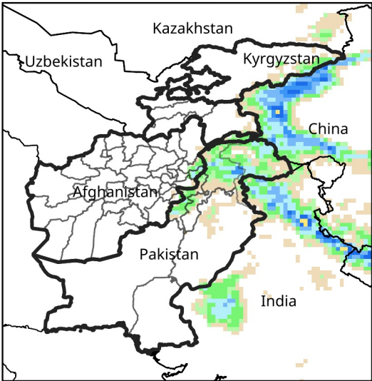
Daily Precip. Forecast for Apr 14, 2025
