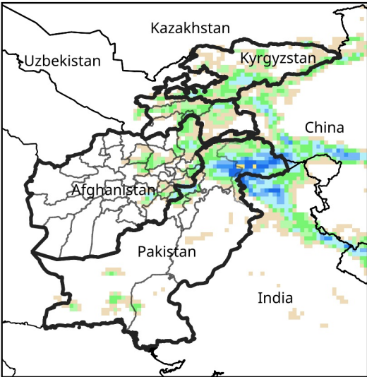
Daily Precip. Forecast for Apr 13, 2025
