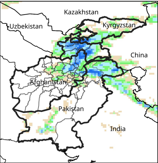
Daily Precip. Forecast for Apr 12, 2025
