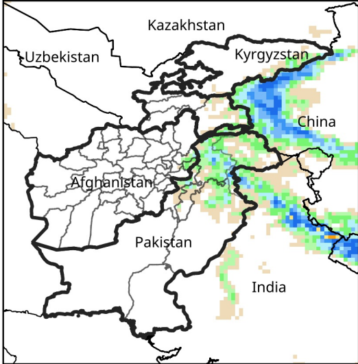
Daily Precip. Forecast for Apr 14, 2025
