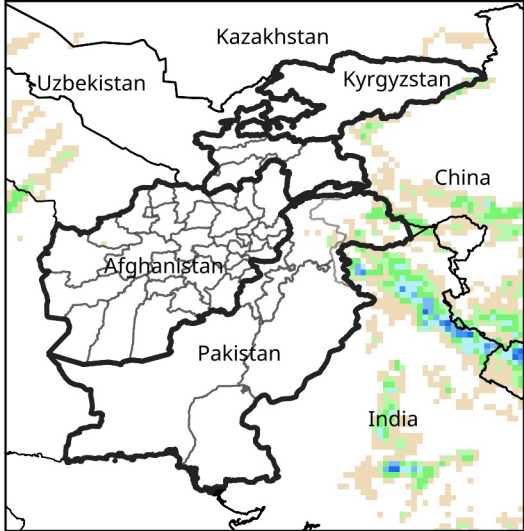
Daily Precip. Forecast for Apr 15, 2025
