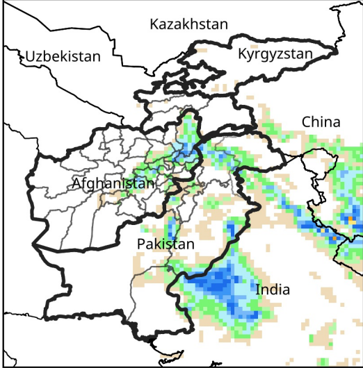
Daily Precip. Forecast for May 4, 2025
