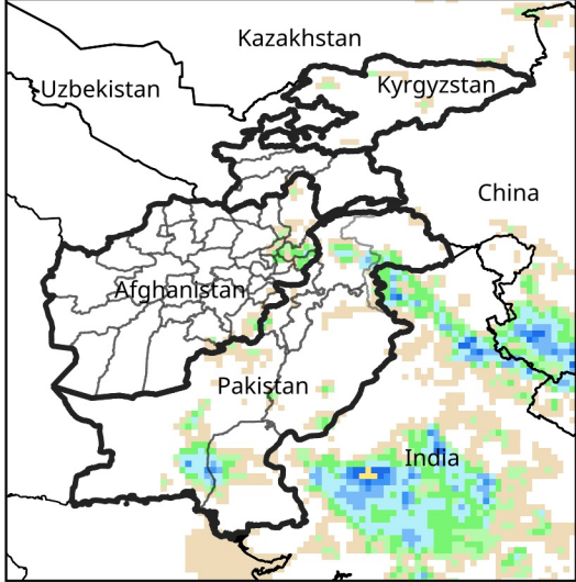
Daily Precip. Forecast for May 5, 2025
