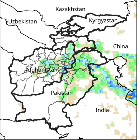
Daily Precip. Forecast for May 3, 2025
