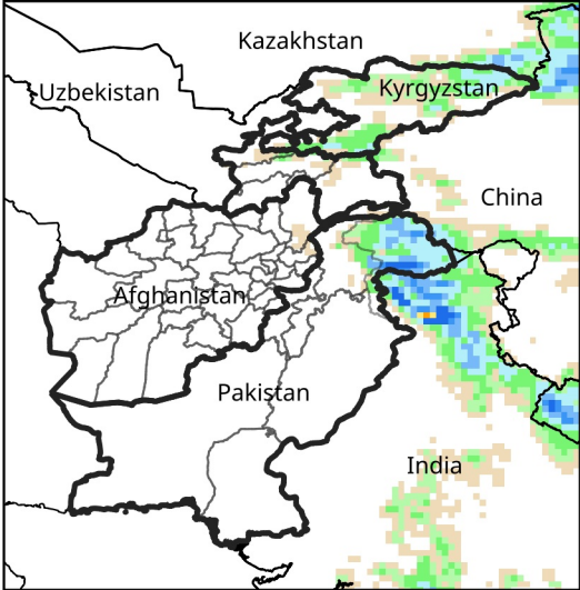
Daily Precip. Forecast for May 22, 2025
