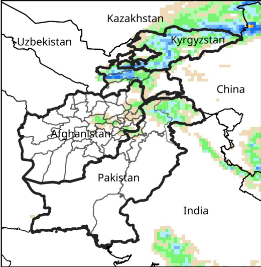
Daily Precip. Forecast for May 21, 2025
