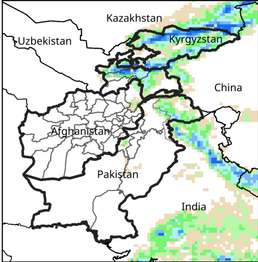
Daily Precip. Forecast for May 23, 2025
