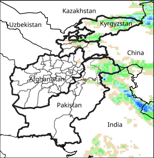
Daily Precip. Forecast for May 22, 2025
