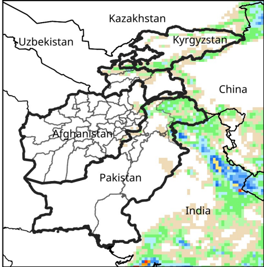
Daily Precip. Forecast for May 24, 2025
