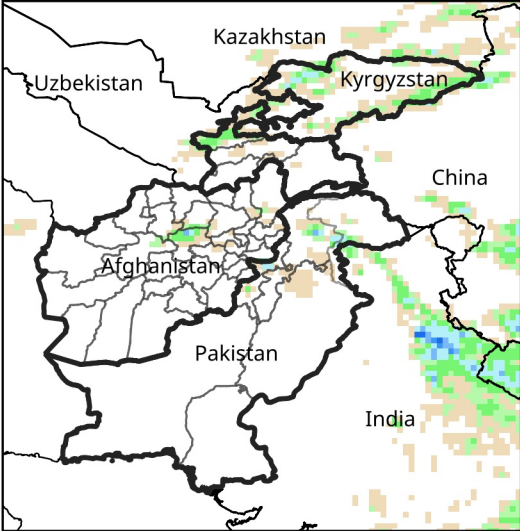
Daily Precip. Forecast for May 28, 2025
