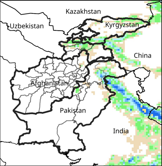
Daily Precip. Forecast for May 27, 2025
