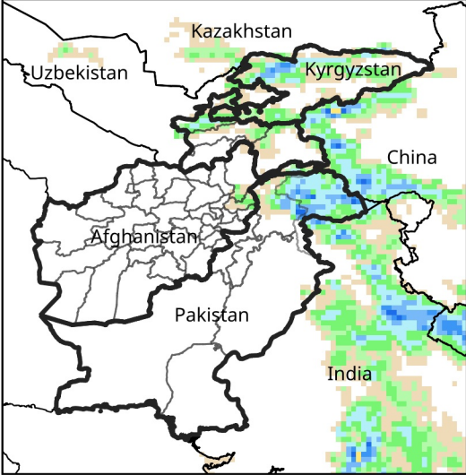
Daily Precip. Forecast for May 28, 2025
