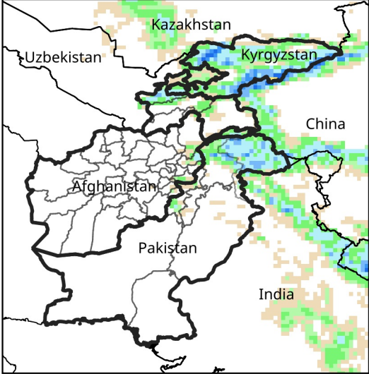
Daily Precip. Forecast for May 29, 2025
