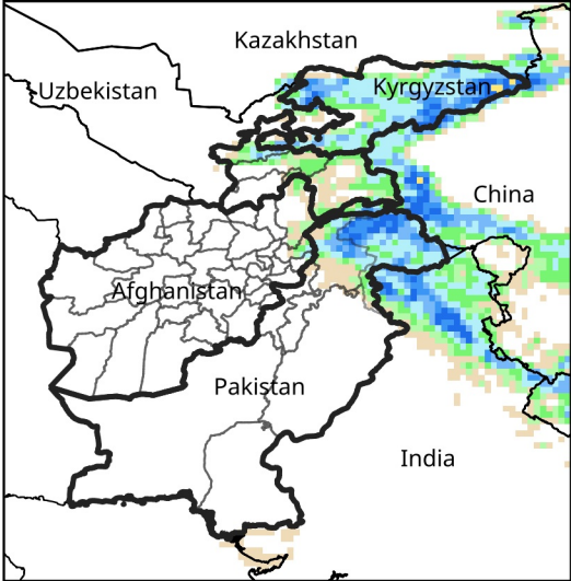
Daily Precip. Forecast for May 31, 2025
