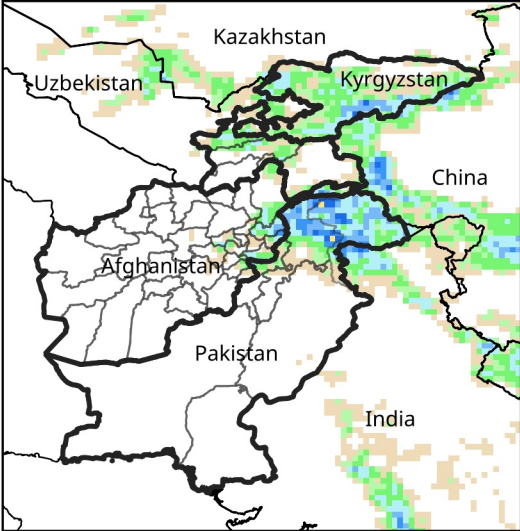
Daily Precip. Forecast for Jun 1, 2025
