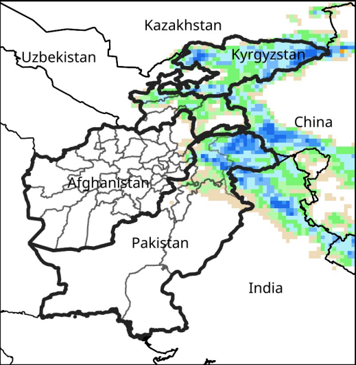
Daily Precip. Forecast for May 31, 2025
