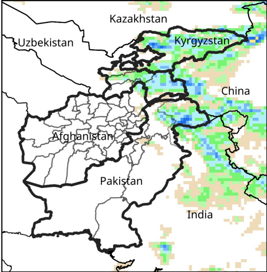
Daily Precip. Forecast for Jun 2, 2025
