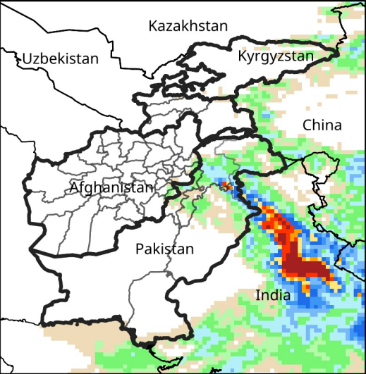
Daily Precip. Forecast for Jun 29, 2025
