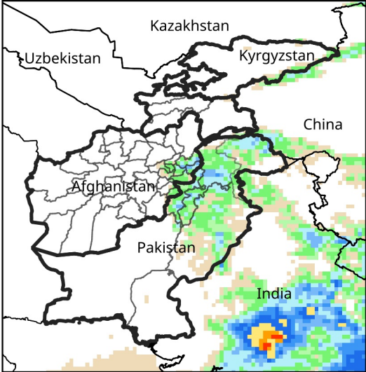
Daily Precip. Forecast for Sep 3, 2025
