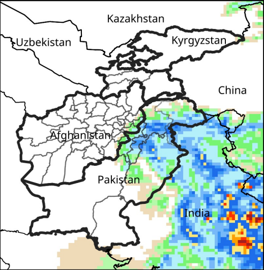
Daily Precip. Forecast for Sep 1, 2025
