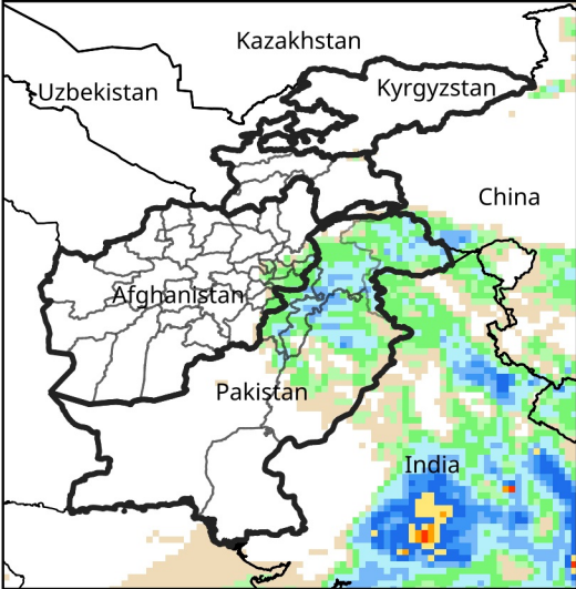
Daily Precip. Forecast for Sep 2, 2025
