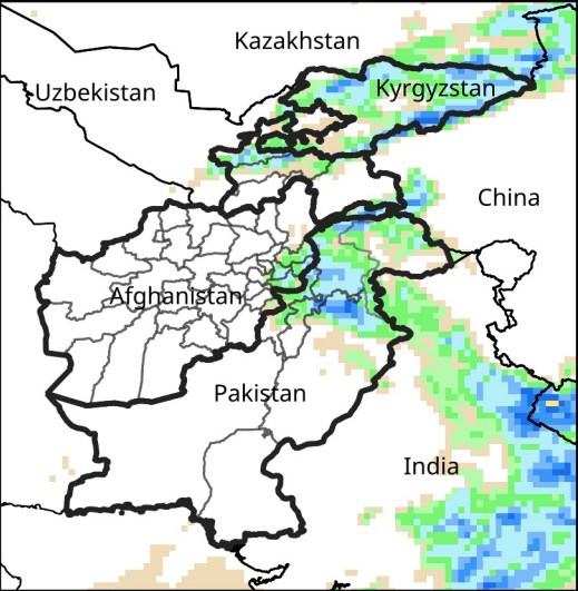
Daily Precip. Forecast for Sep 21, 2025
