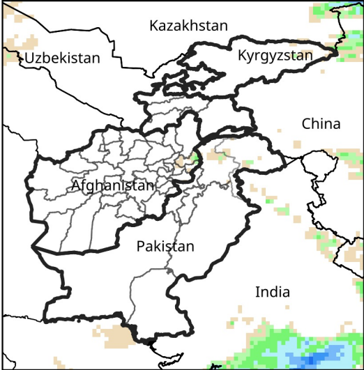
Daily Precip. Forecast for Sep 23, 2025
