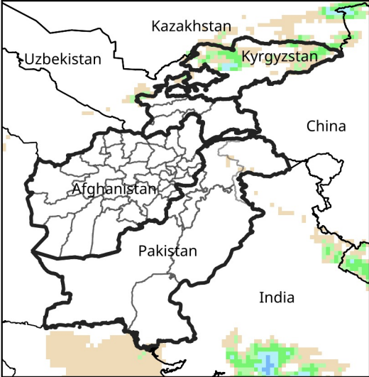
Daily Precip. Forecast for Sep 22, 2025
