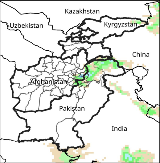
Daily Precip. Forecast for Sep 24, 2025
