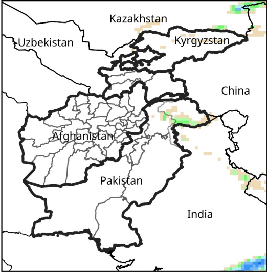
Daily Precip. Forecast for Oct 18, 2025
