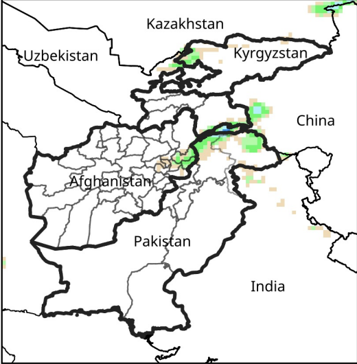
Daily Precip. Forecast for Oct 19, 2025
