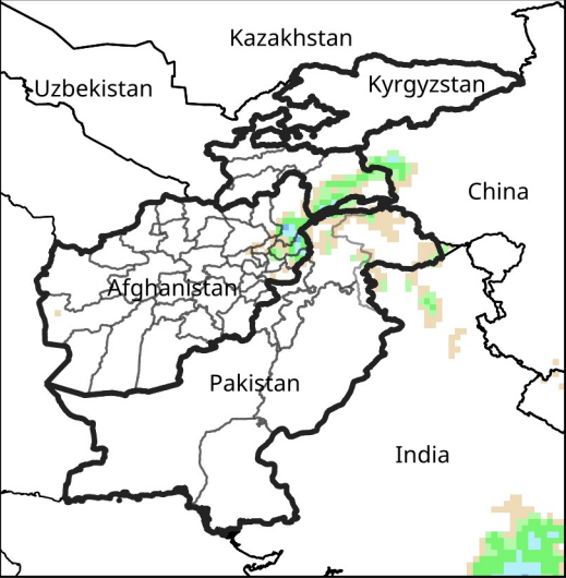
Daily Precip. Forecast for Oct 21, 2025
