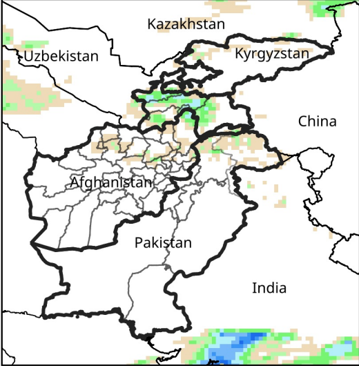
Daily Precip. Forecast for Oct 27, 2025
