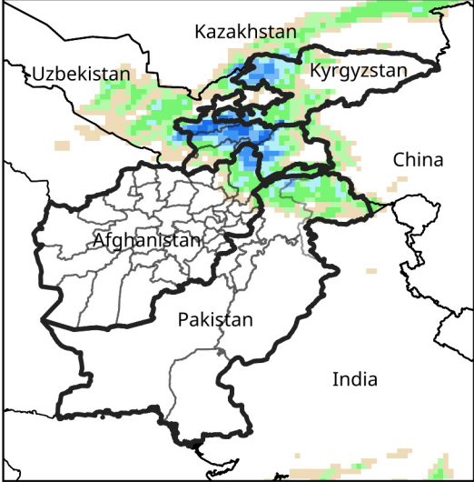
Daily Precip. Forecast for Oct 28, 2025
