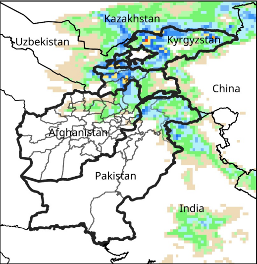
Daily Precip. Forecast for Nov 7, 2025
