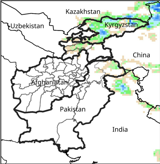
Daily Precip. Forecast for Nov 8, 2025
