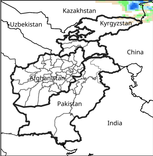
Daily Precip. Forecast for Nov 16, 2025
