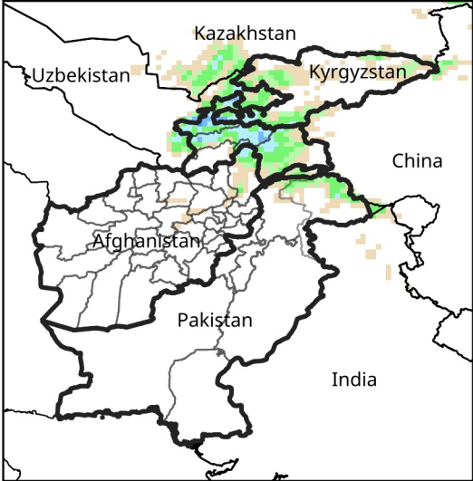
Daily Precip. Forecast for Dec 8, 2025
