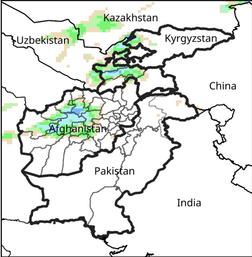
Daily Precip. Forecast for Dec 7, 2025
