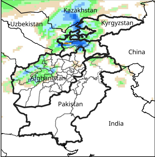
Daily Precip. Forecast for Dec 14, 2025
