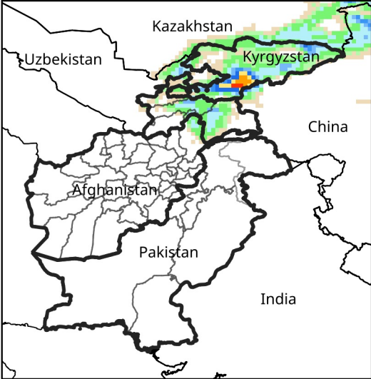
Daily Precip. Forecast for Dec 13, 2025
