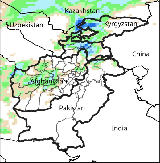
Daily Precip. Forecast for Dec 14, 2025
