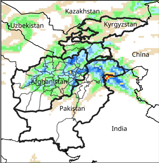
Daily Precip. Forecast for Dec 24, 2025
