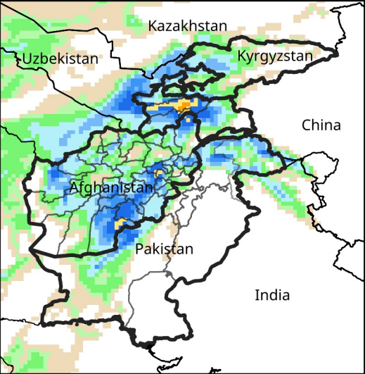
Daily Precip. Forecast for Dec 23, 2025
