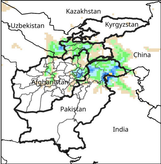
Daily Precip. Forecast for Dec 25, 2025
