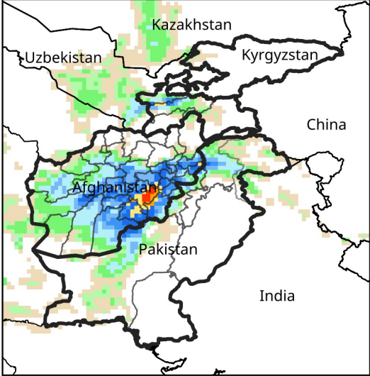
Daily Precip. Forecast for Dec 30, 2025
