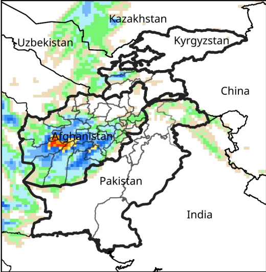
Daily Precip. Forecast for Jan 1, 2026
