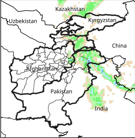
Daily Precip. Forecast for Jan 1, 2026
