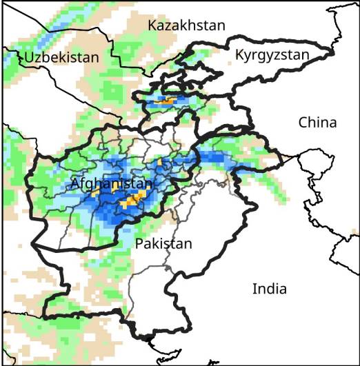
Daily Precip. Forecast for Jan 2, 2026
