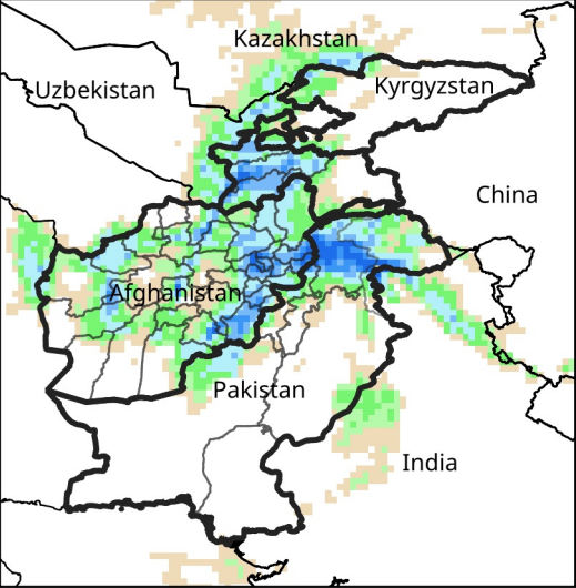
Daily Precip. Forecast for Dec 31, 2025
