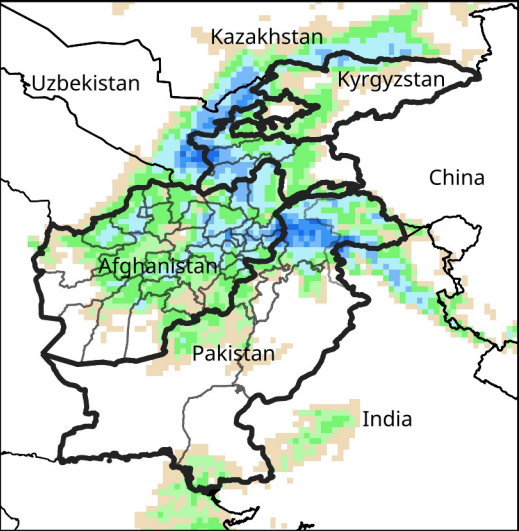
Daily Precip. Forecast for Jan 3, 2026
