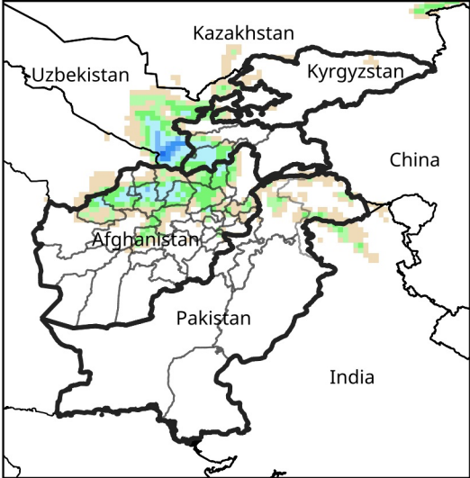
Daily Precip. Forecast for Jan 5, 2026
