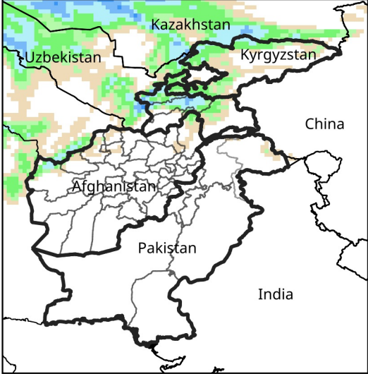
Daily Precip. Forecast for Jan 15, 2026
