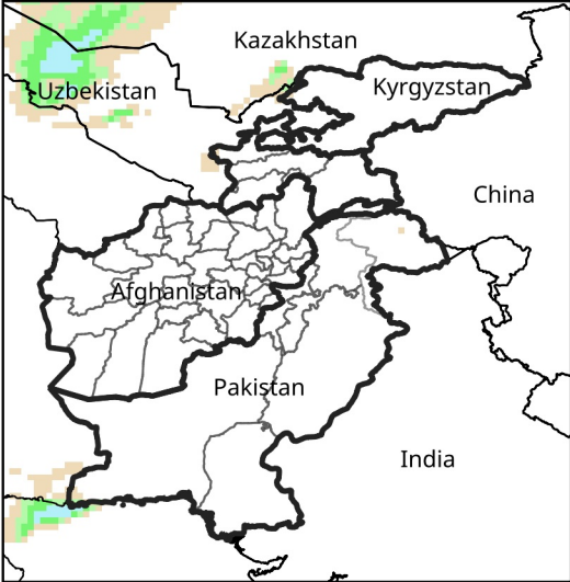
Daily Precip. Forecast for Jan 14, 2026
