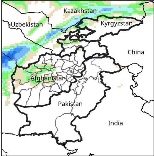
Daily Precip. Forecast for Jan 18, 2026
