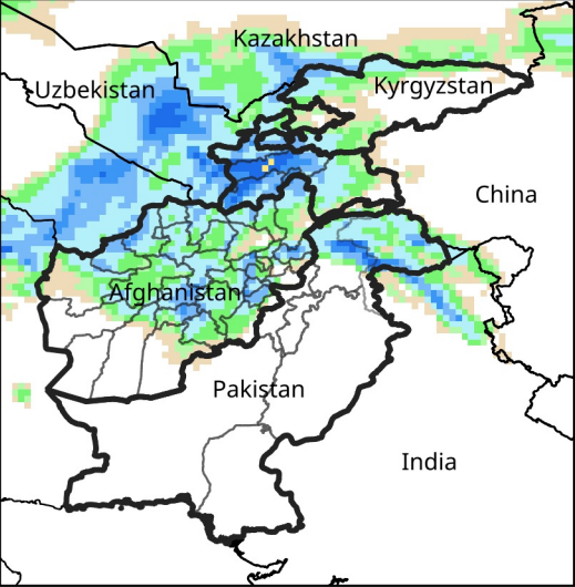
Daily Precip. Forecast for Jan 16, 2026
