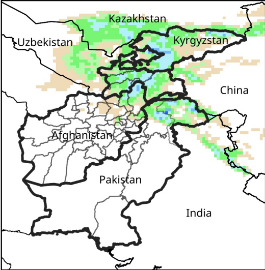
Daily Precip. Forecast for Jan 20, 2026
