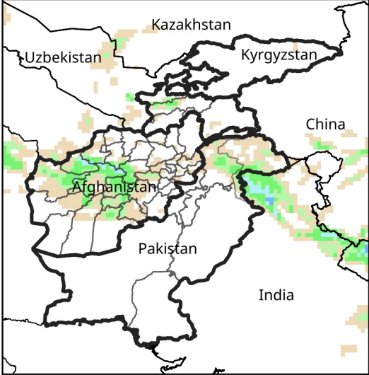
Daily Precip. Forecast for Jan 24, 2026
