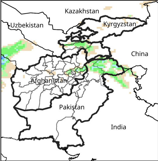
Daily Precip. Forecast for Jan 23, 2026
