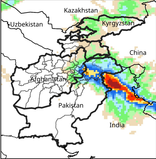
Daily Precip. Forecast for Jan 23, 2026
