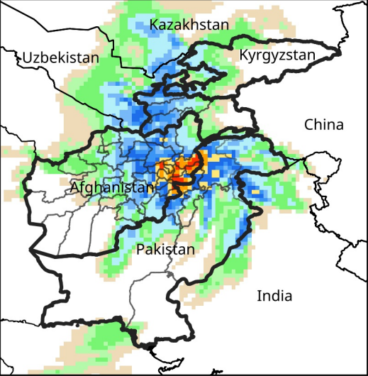
Daily Precip. Forecast for Jan 22, 2026
