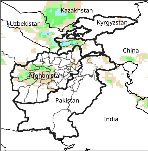
Daily Precip. Forecast for Jan 27, 2026
