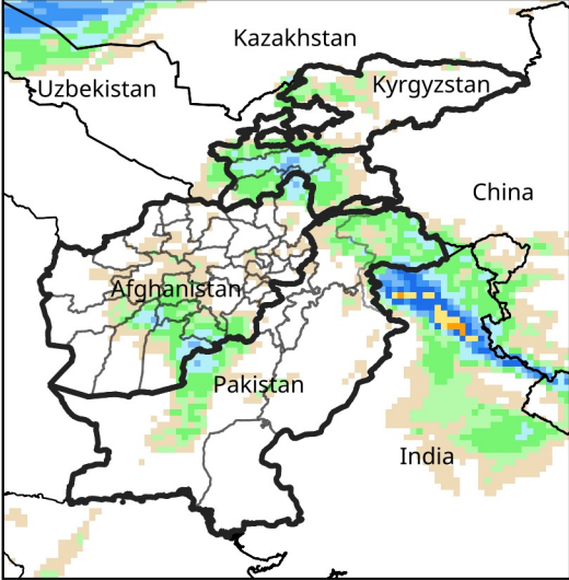
Daily Precip. Forecast for Jan 27, 2026
