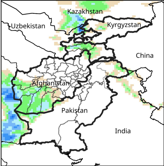
Daily Precip. Forecast for Jan 28, 2026
