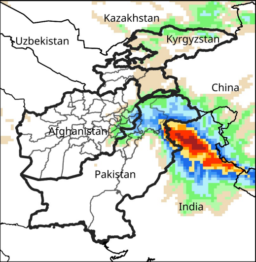
Daily Precip. Forecast for Jan 26, 2026
