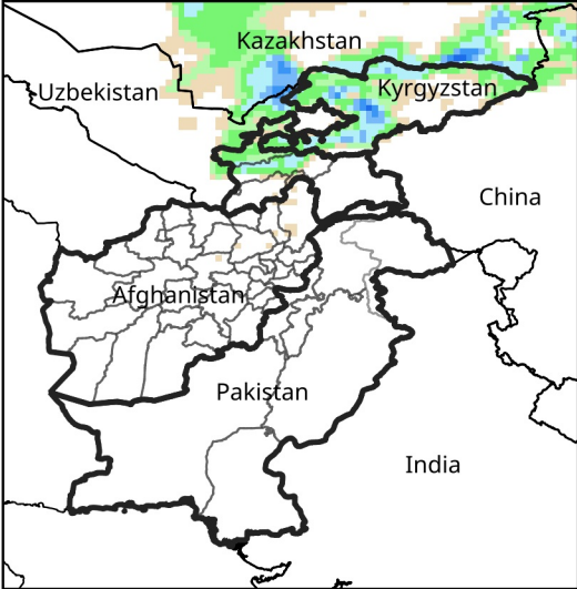
Daily Precip. Forecast for Feb 21, 2026
