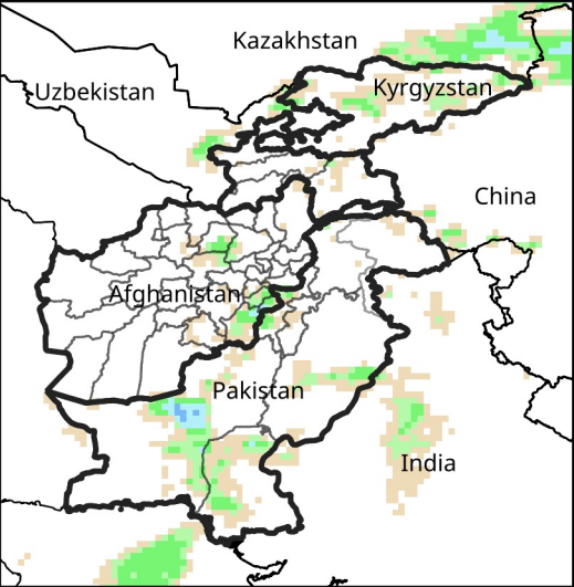
Daily Precip. Forecast for Feb 20, 2026
