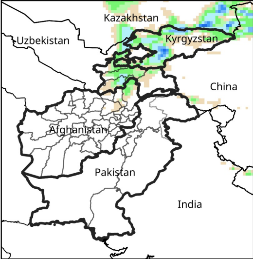
Daily Precip. Forecast for Feb 24, 2026
