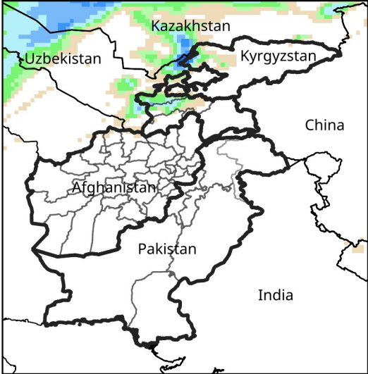
Daily Precip. Forecast for Feb 25, 2026
