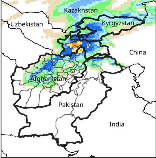
Daily Precip. Forecast for Mar 5, 2026
