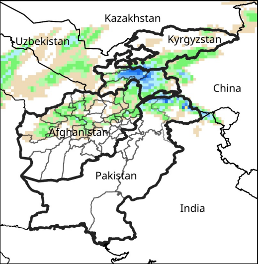
Daily Precip. Forecast for Mar 6, 2026
