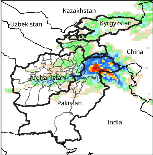
Daily Precip. Forecast for Mar 11, 2026
