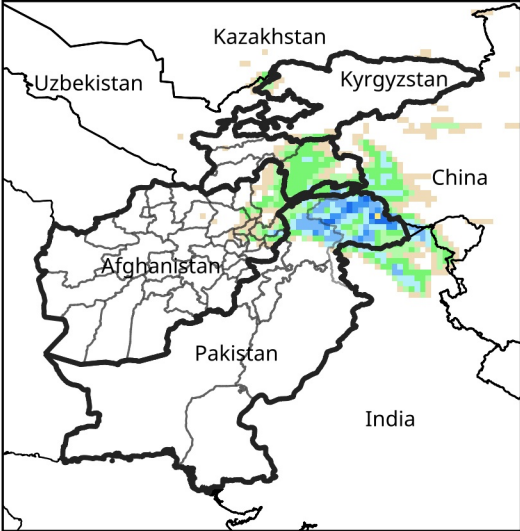
Daily Precip. Forecast for Mar 10, 2026
