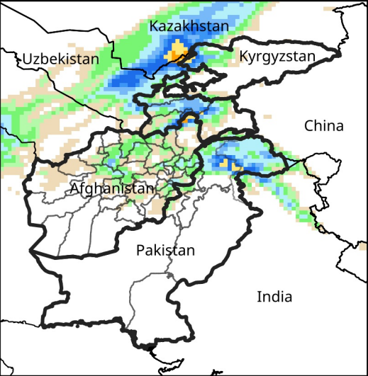
Daily Precip. Forecast for Mar 9, 2026
