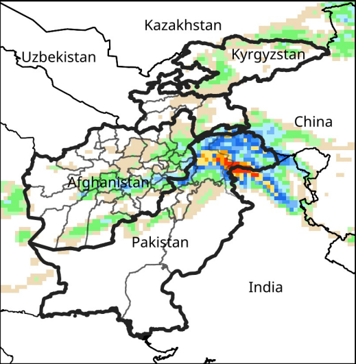
Daily Precip. Forecast for Mar 11, 2026
