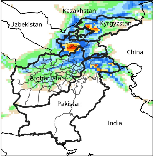
Daily Precip. Forecast for Mar 13, 2026
