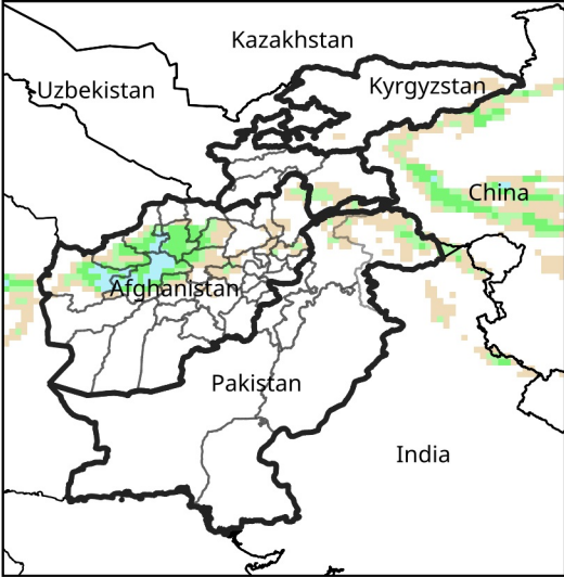
Daily Precip. Forecast for Mar 13, 2026
