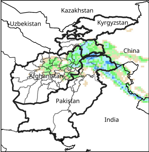
Daily Precip. Forecast for Mar 14, 2026
