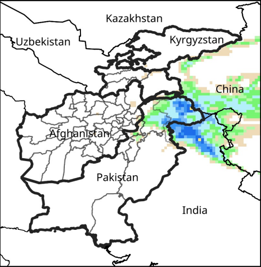
Daily Precip. Forecast for Mar 12, 2026
