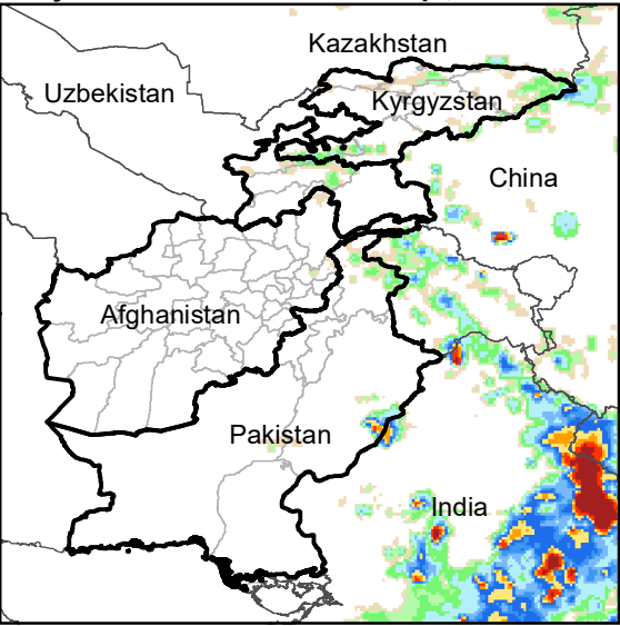
Daily Rainfall estimate for 5 Sep., 2002
